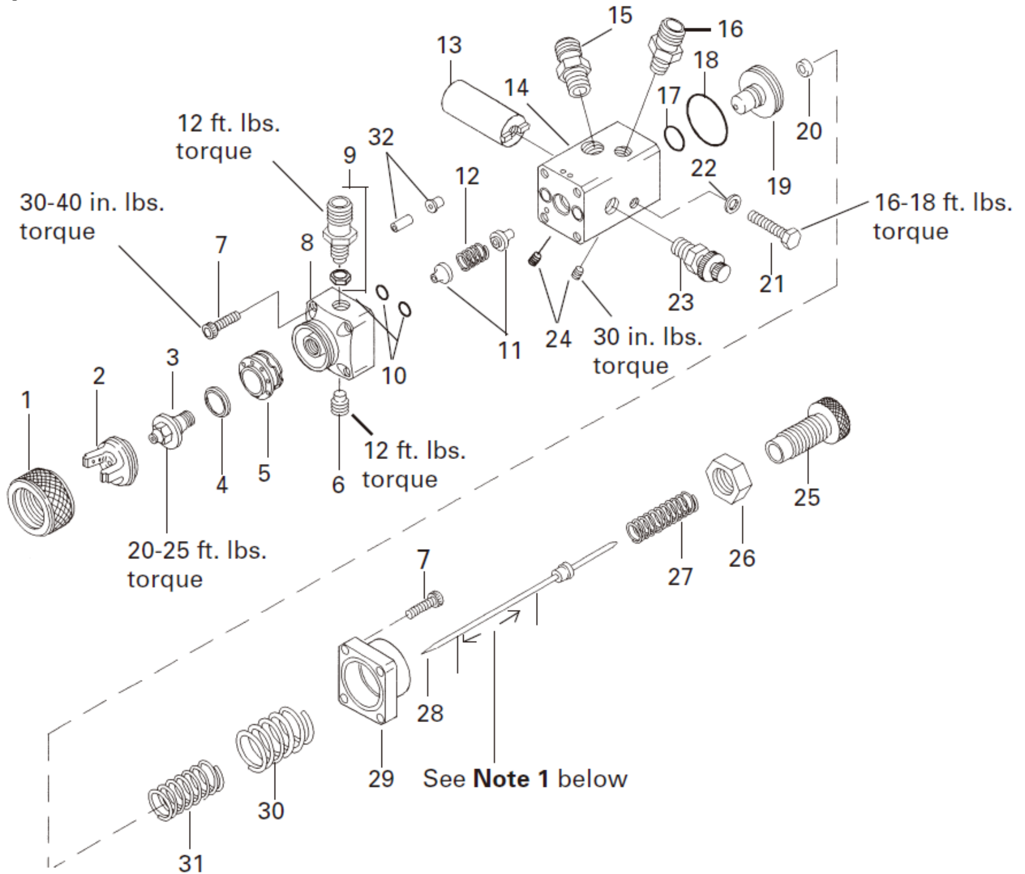
Figure 4 GUN ASSEMBLY
