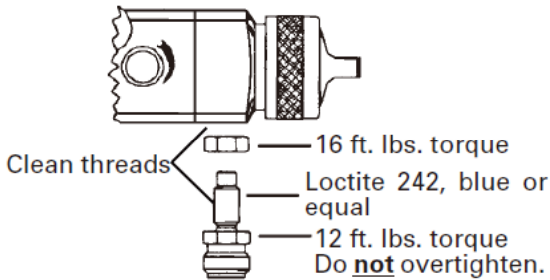
Figure 5. Gun Exploded View
