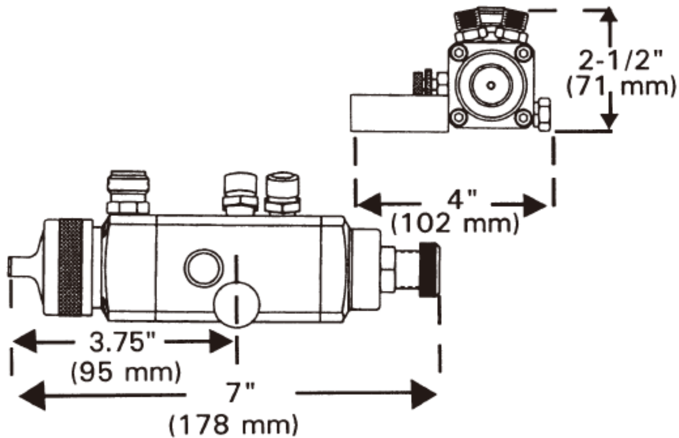
FIGURE 1 DIMENSIONS
